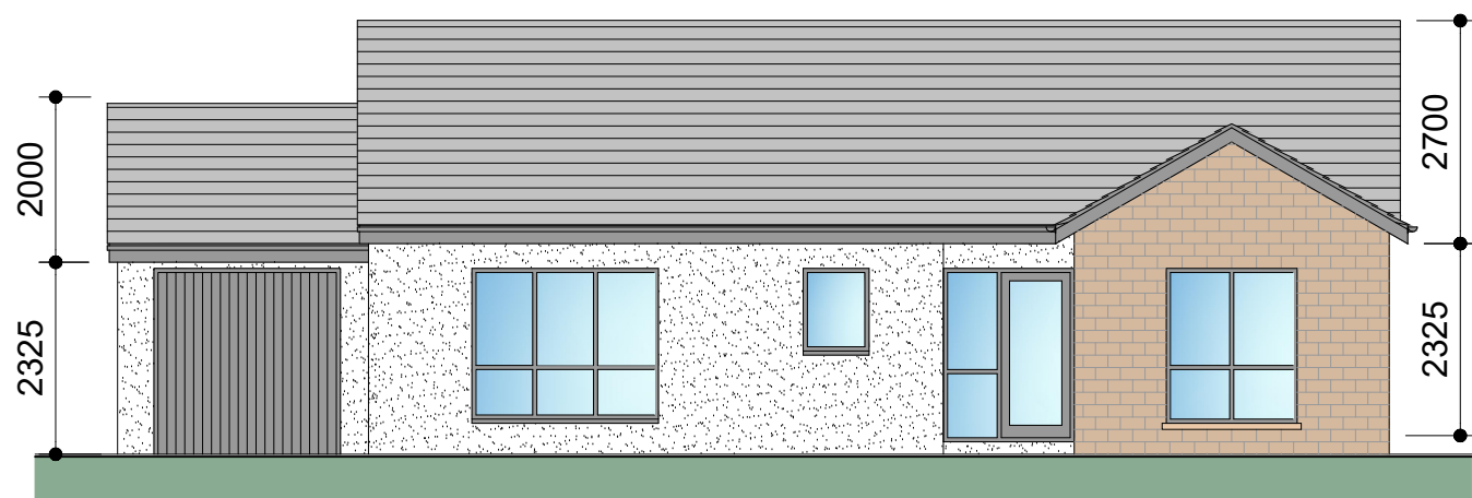
Front Elevation
