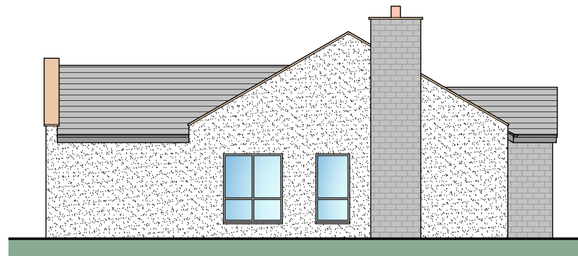
Side Elevation
