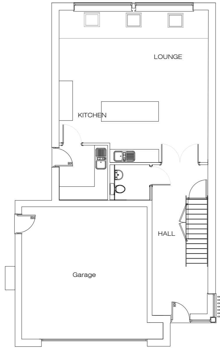
Ground Floor Scale 1:50
