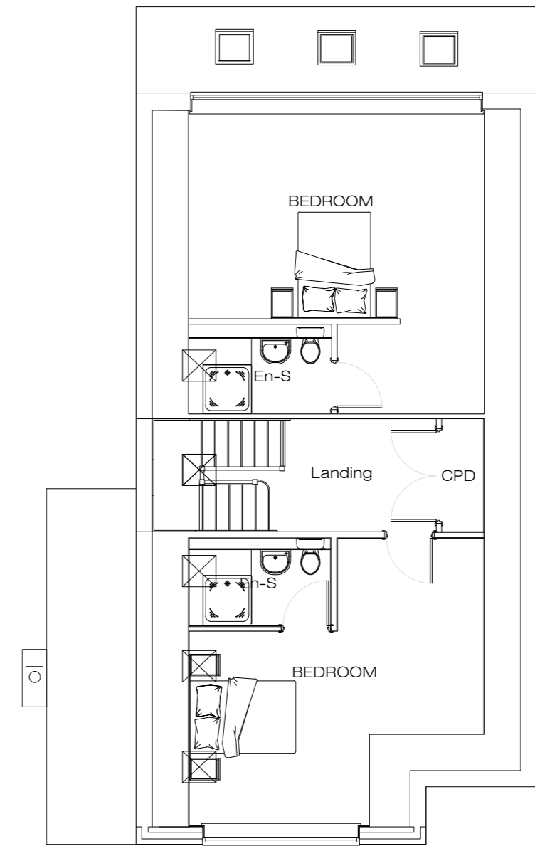
Second Floor Scale 1:50
