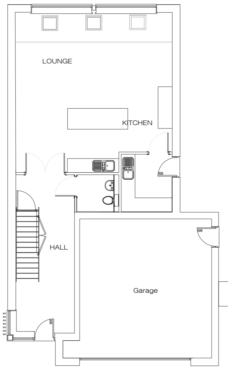
Ground Floor Scale 1:50
