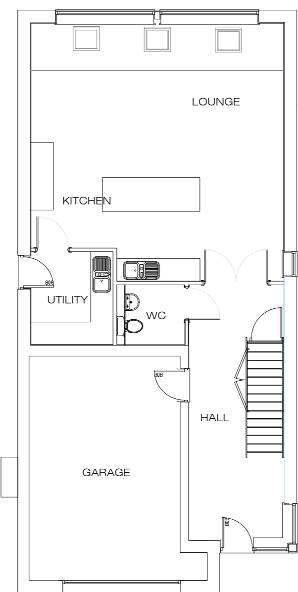
Ground Floor Scale 1:50
