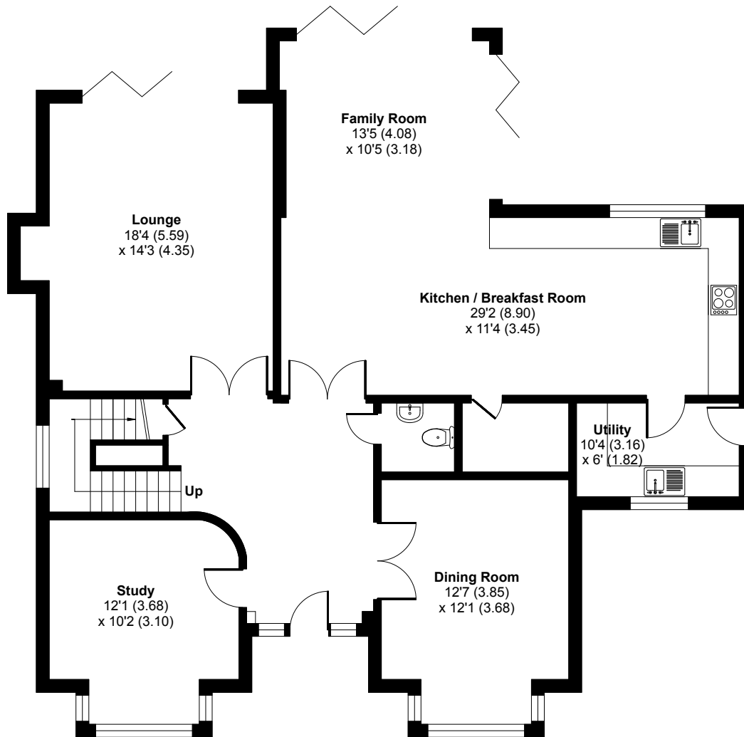
GROUND FLOOR
